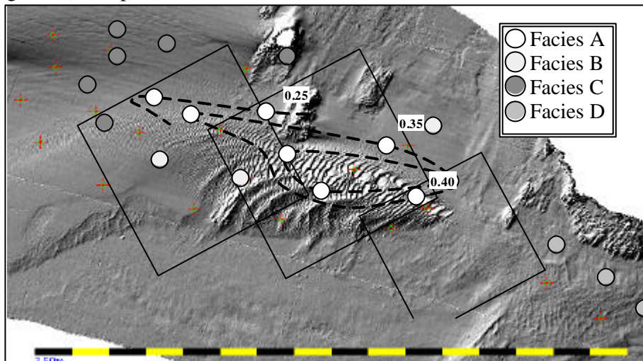
Figure 3SEQARABE Facies locations and ADCP tracks taken. Grain size contour lines are also shown (units in mm)
