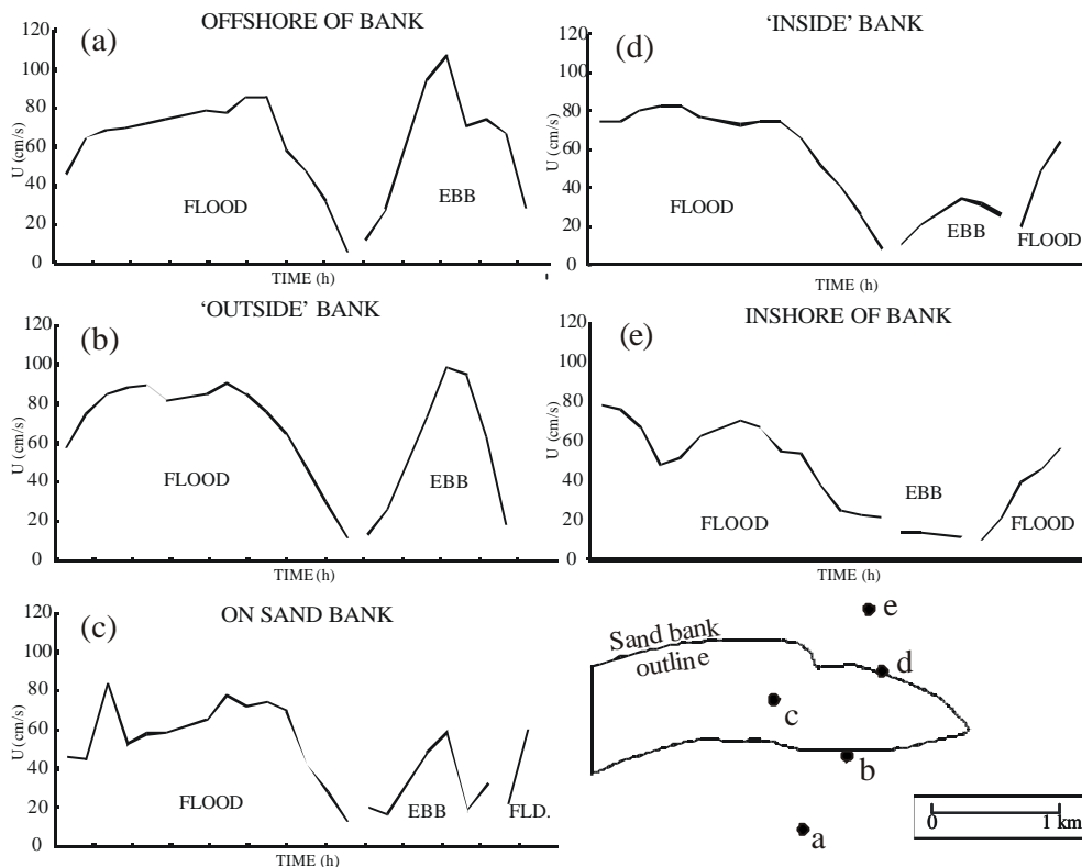
Figure 7SEQARABE Plot showing increasing flood domination of depth averaged currents from offshore of sand bank (plot a) to inshore of sand bank (plot e)
