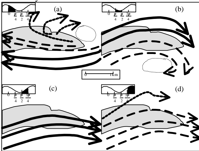
Figure 5SEQARABE Interpretation of depth averaged current vectors. The ‘snapshots’ are based on current vectors averaged over 3 hours of the tidal cycle. The outline of the sand bank is depicted by the dotted area.
