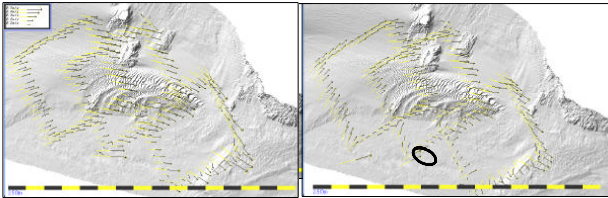
Figure 9 Residual currents across the sand bank. LEFT: Depth averaged; RIGHT: Bottom 10 m averaged currents
