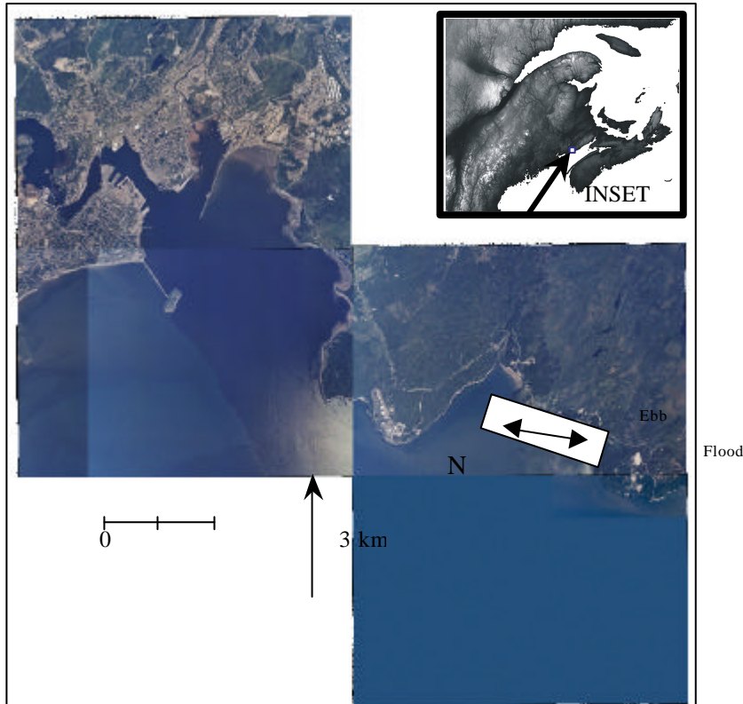
Figure 1: SEQARABE: Location Map. Saint John, New Brunswick is shown in the upper left part of the picture and the field area is depicted by the white rectangle. Ebb and flood directions are also depicted. The headland, Cape Spencer, is on the extreme right.
