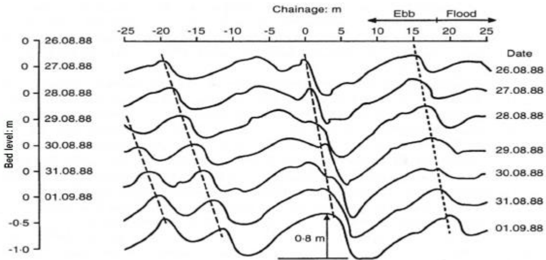
Figure 1 Sandwave migration in a sandy estuary (from Soulsby, 1997), by permission of Thomas Telford Ltd, London
