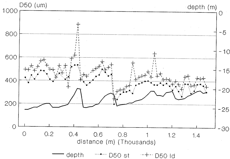
Fig.5 Morphology and grainsize of profile Z1. Grainsize is determined by settling tube (D50 st) and by laser diffraction (D50 ld)
