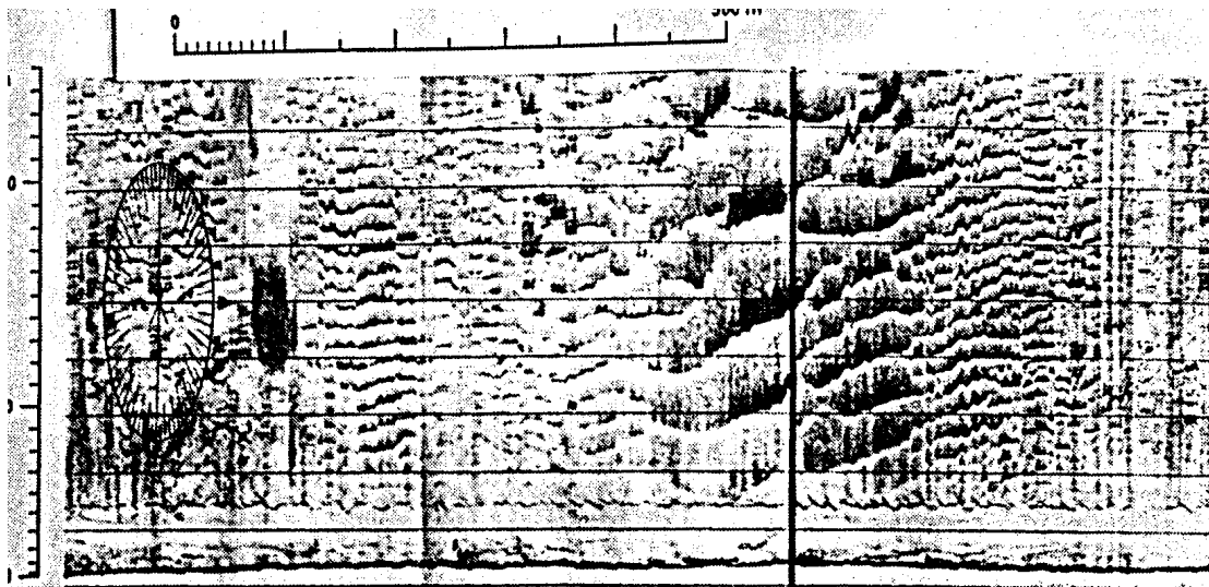
Fig. 2. Coexistence of different dune size hierarchies along lateral, cross-flow velocity gradients. Note the quasi-symmetrical arrangement of individual size hierarchies, the relatively sharp boundaries between adjacent dune trains, and the absence of smaller superimposed dunes in each case (flow direction from bottom to top).
