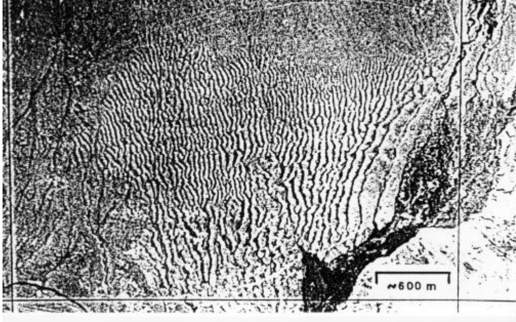
Fig. 3. Air photo of large gravel dunes produced by a catastrophic glacial outflow event in the Altai Mountains of Siberia (from Carling, 1996). The flow is from right to left. Note the hierarchical pattern of different dune sizes in both the downstream and cross-flow directions.
