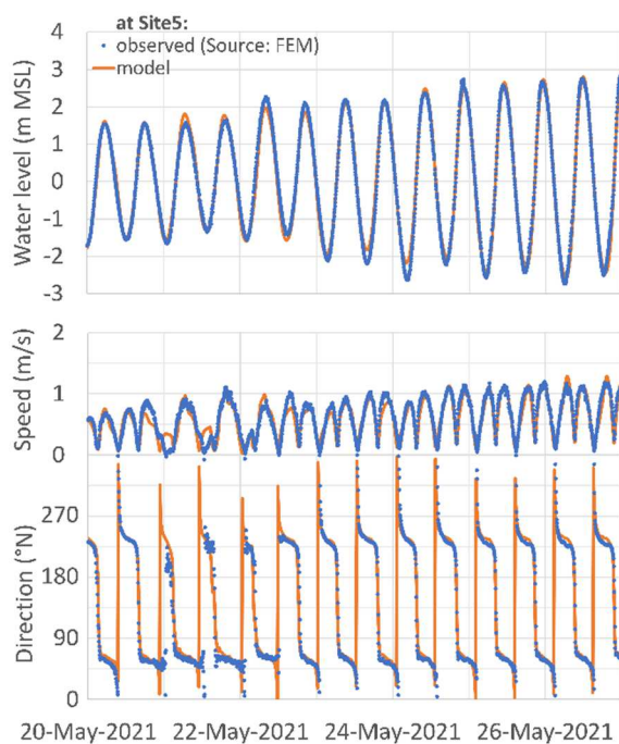
Figure 3. Comparison of model predictions against observed tidal levels (top), current magnitude (centre) and direction (bottom) for a 7-day period in 2021.
